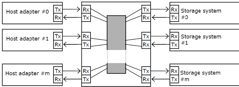
(b) Fibre Channel Switch Connection
