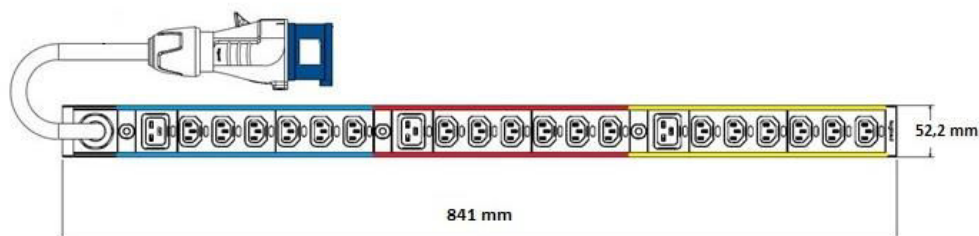
Figure 7 APAC and EMEA PDU for the Hitachi Universal V2B Rack (Single-phase 1P32A-18C13-3C19CE.P)
