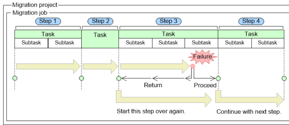
Figure 2 Example of failed migration task
