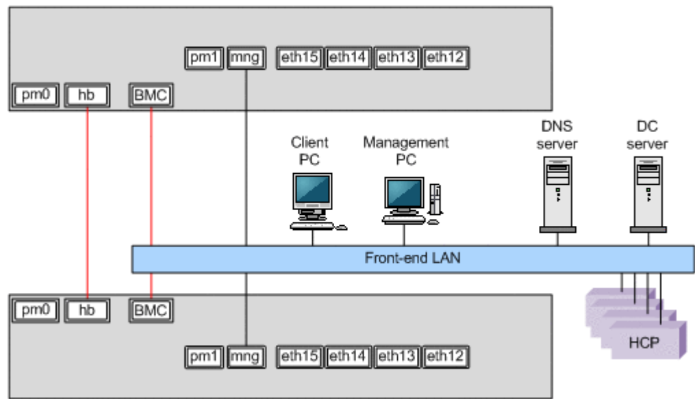
Figure 1-1 Network configuration
