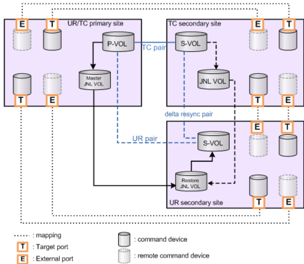
Figure 4 Remote command devices in a delta resync configuration
